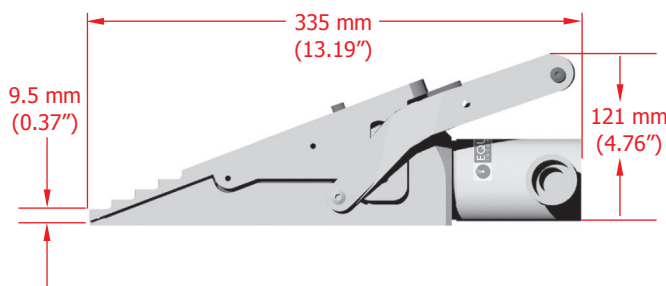
TOOL DIMENSIONS - CLOSED
